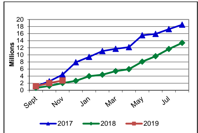
Figure 4: Assessed Penalties
