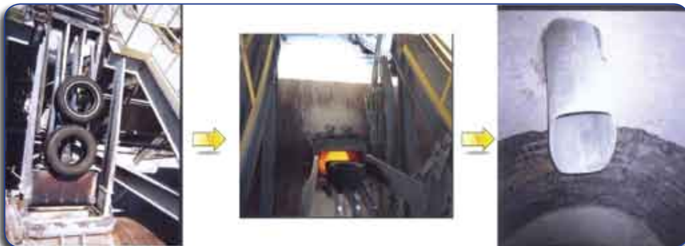
Exhibit 4-2. Mid-kiln injection Source: North Texas Cement
